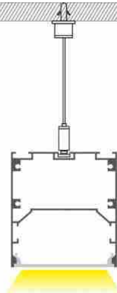
悬挂式安装 Hanging installation
