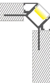
阳角嵌入式安装 Angle Embedded Installation
