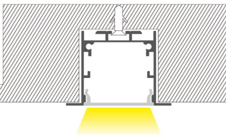
嵌入式安装 Embedded installation
