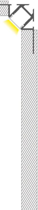
阴角嵌入式安装 Inner angle embedded installation
