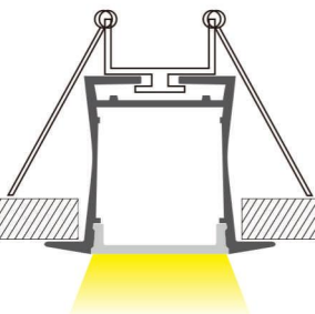
嵌入式安装 Embedded installation
